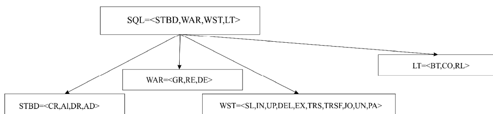
Fig. 2. Affiliation graf for structured language SQL
